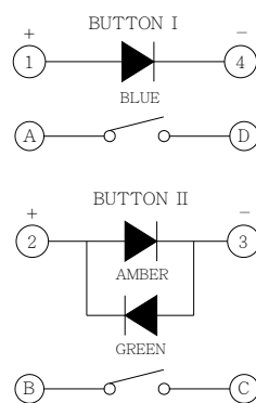
CIRCUIT DIAGRAM
