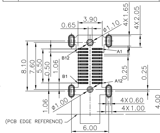
RECOMMENDED P.C.B LAYOUT TOLERANCE ± 0.05mm (TOP VIEW)
