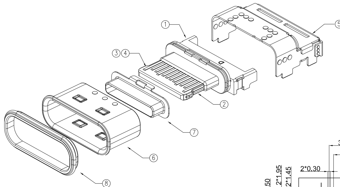
Explode View
